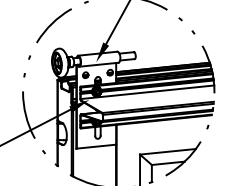
LOW HEADROOM TRACK DETAIL F
